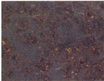
Mill scale has started to flake, light rusting occurs
